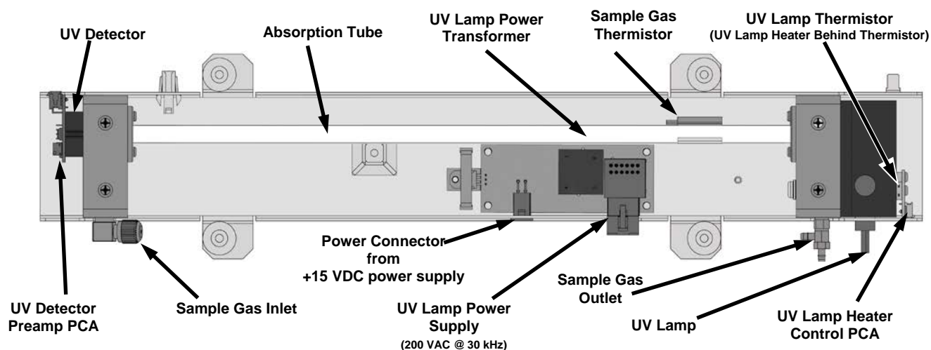
Figure 9-23: O 3 Photometer Layout – Top Cover Removed
