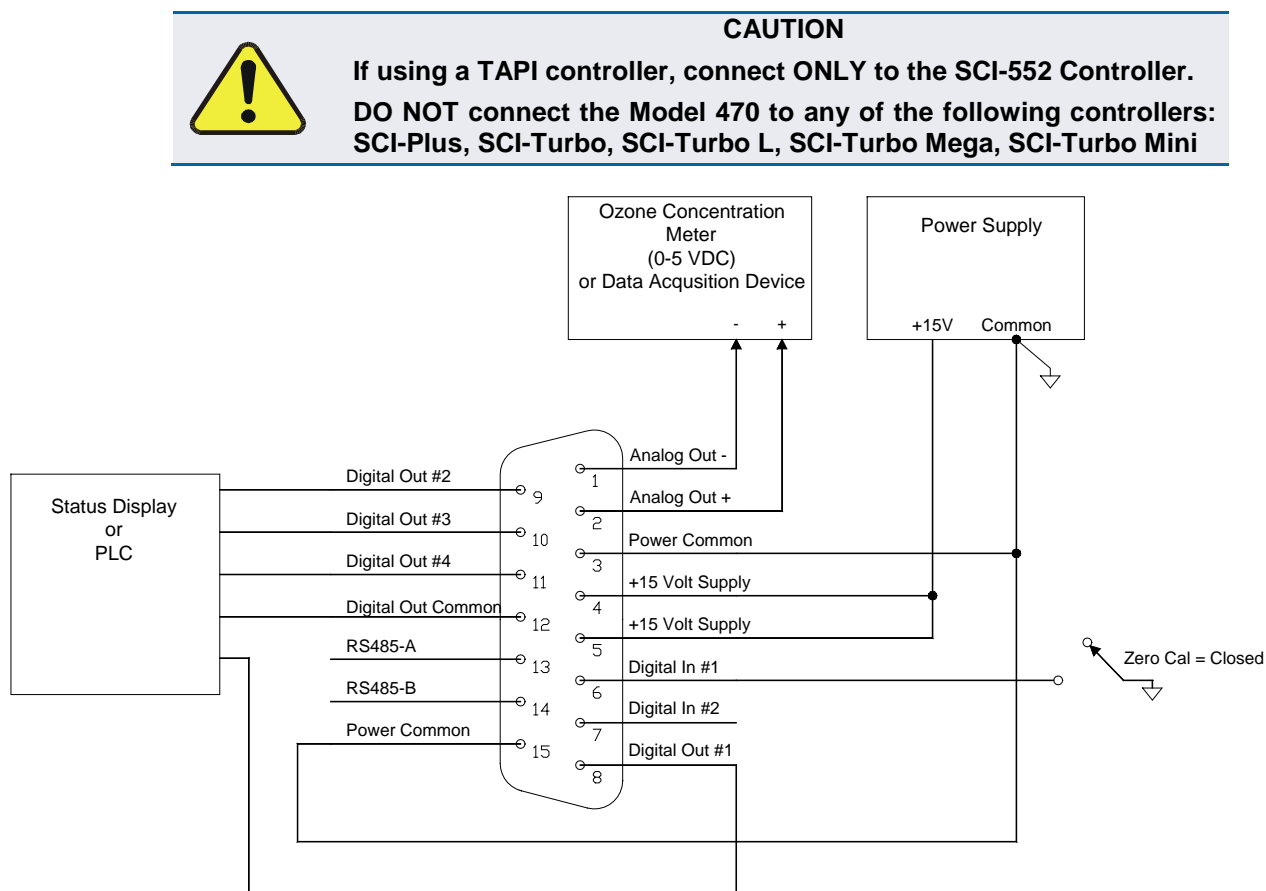
Figure 2-5: Digital Output Connections
