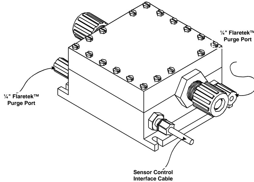
Figure 2-1. Sensor Diagram
