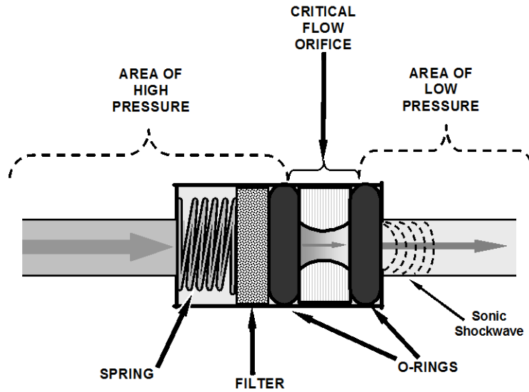
Figure 12-6: Flow Control Assembly & Critical Flow Orifice
