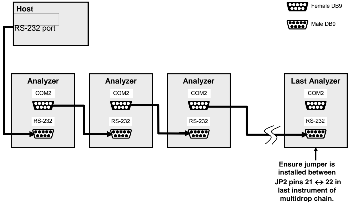
Figure 3-15: RS-232-Multidrop PCA Host/Analyzer Interconnect Diagram
