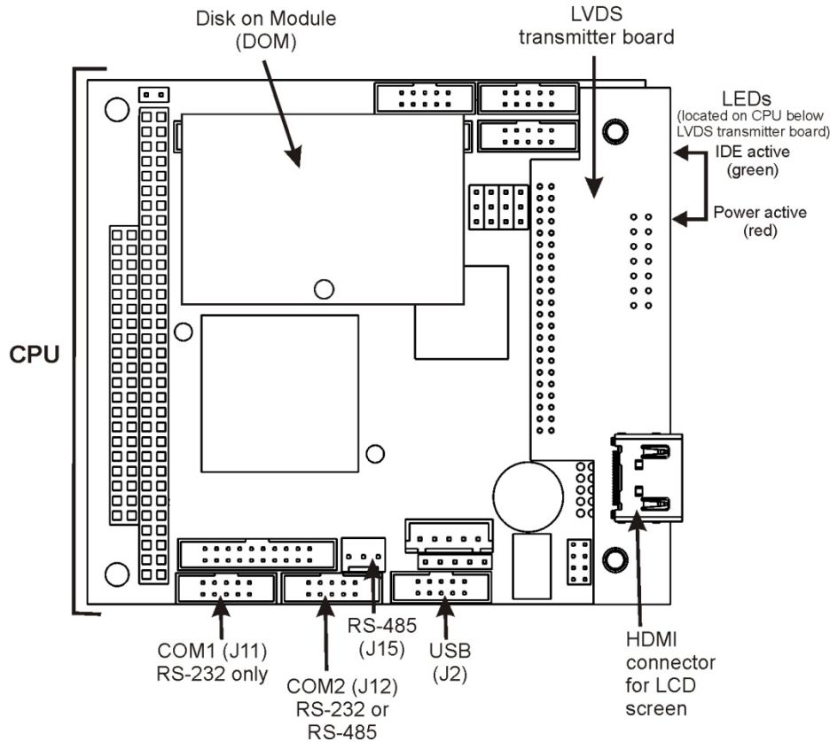
Figure 12-8. CPU Card
