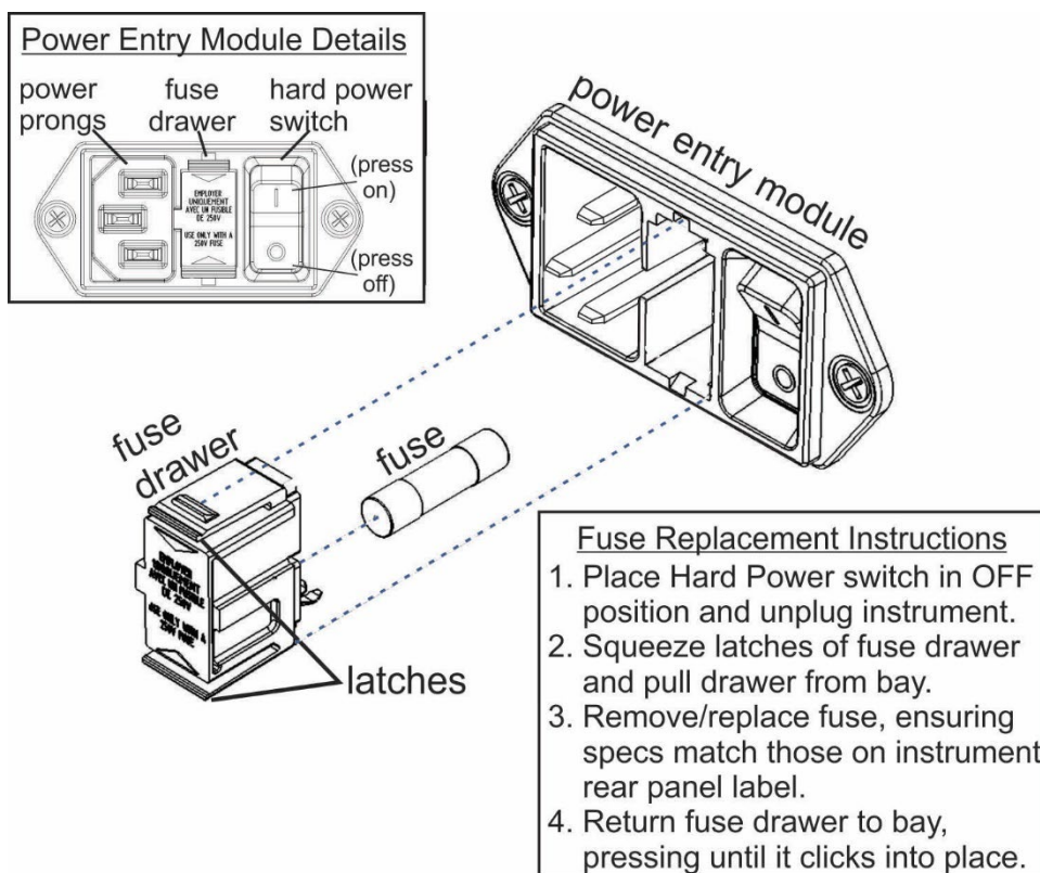
Figure 5-12. Fuse Access
